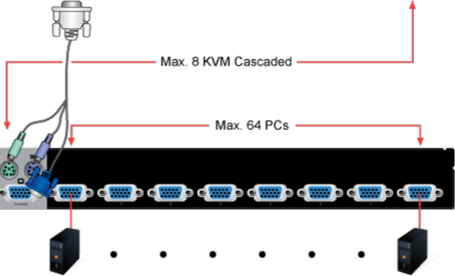
KVM-210-08M Rear Panel
