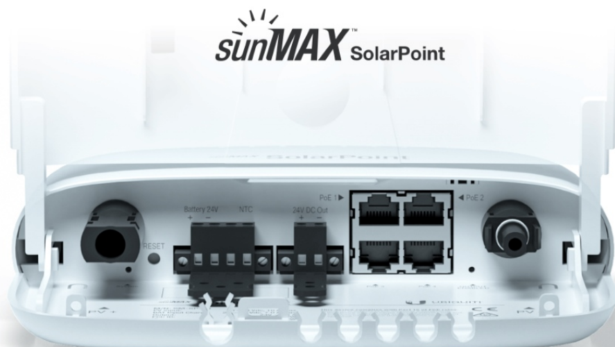
PV Panel Terminal Battery Terminal Power Terminal Ethernet Ports PV Panel Terminal
