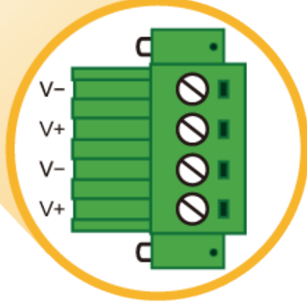
4-pin DC Power Input Connector
